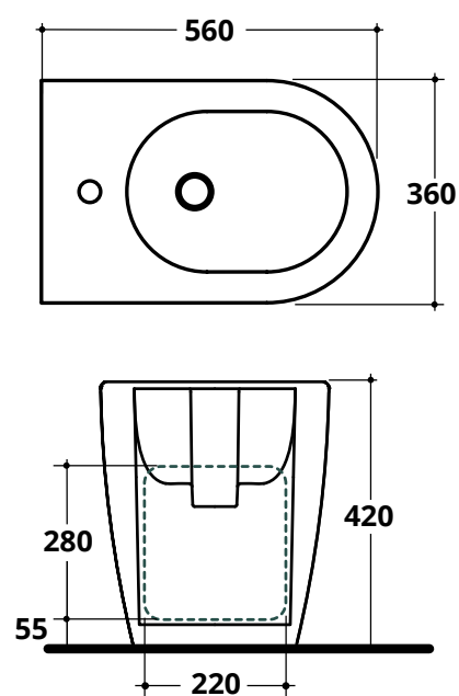
COVER XL Bidet TRASLATO H. 42 cm ADJUSTABLE INSTALLATION COD. AS011
