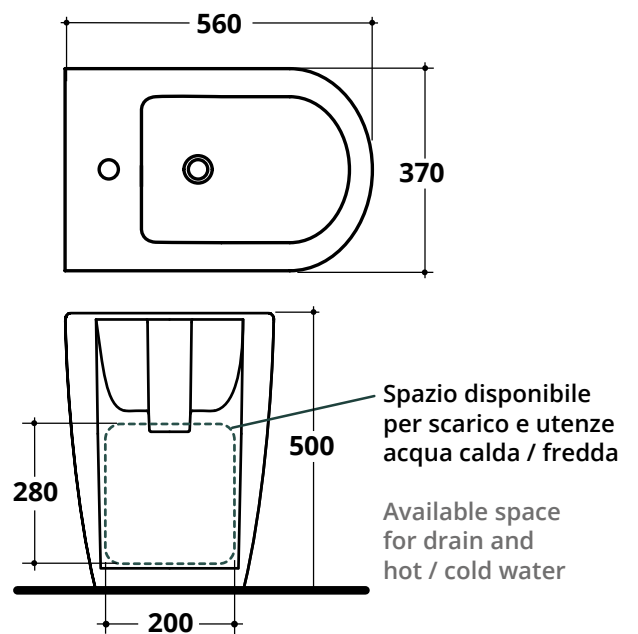
COVER XL Bidet TRASLATO H. 50 cm ADJUSTABLE INSTALLATION
