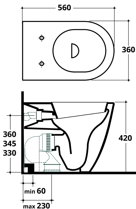
COVER XL WC TRASLATO H. 42 cm ADJUSTABLE INSTALLATION COD. AS010
