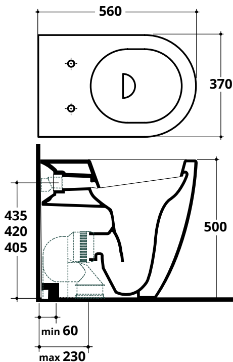
COVER XL WC TRASLATO H. 50 cm ADJUSTABLE INSTALLATION
